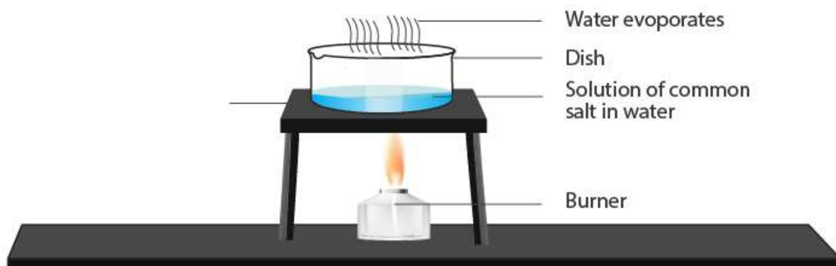
Seperation of common salt dissolved in water by evaporation
