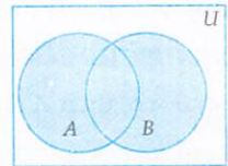
Fig. 1.6 Union of two sets
