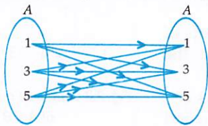
Fig. 2.8 Arrow diagram of A \times A
