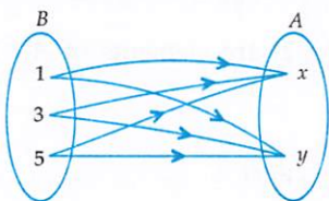
Fig. 2.6 Arrow diagram of A \times B
